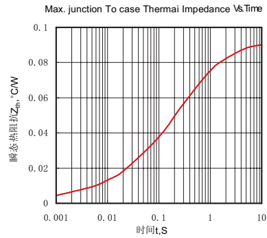
Fig.2 瞬态热阻抗抗曲线
