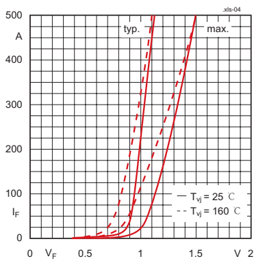
Fig. 5 Forward characteristics
